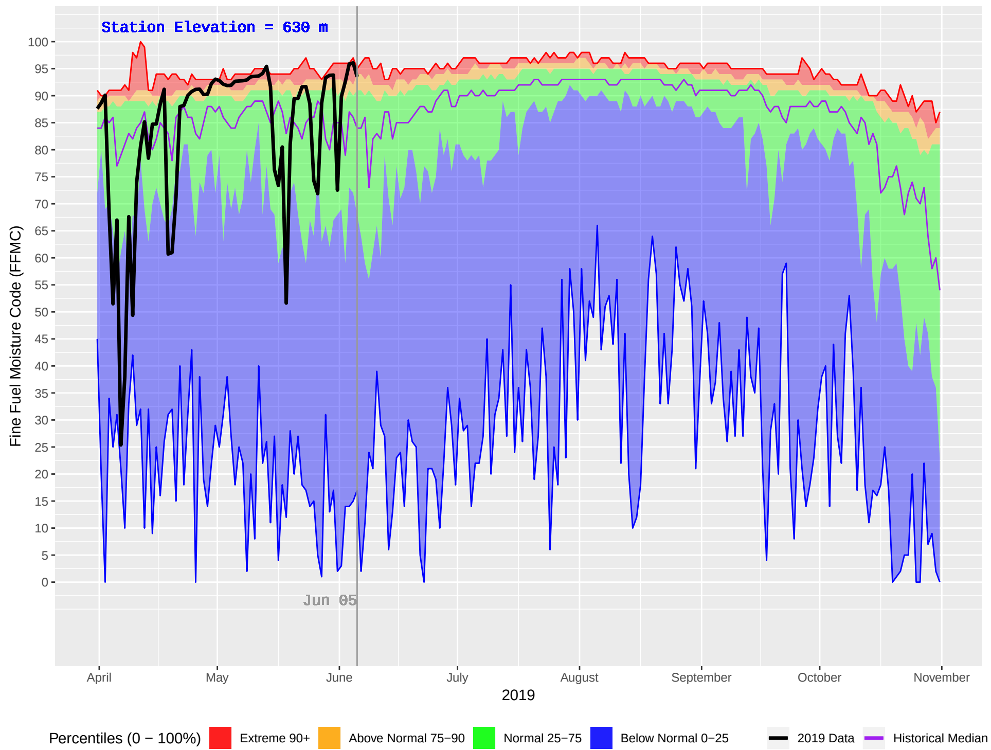
GRAND FORKS (392) : Historical (1981–2018) and Current (2019) Daily Fine Fuel Moisture Code (FFMC)
