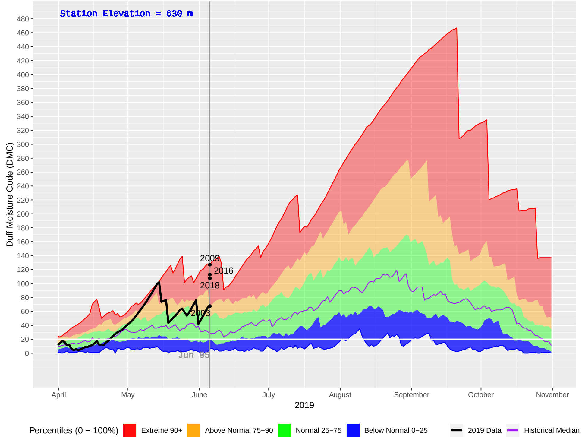
GRAND FORKS (392) : Historical (1981–2018), Current (2019) Daily Duff Moisture Code (DMC)
