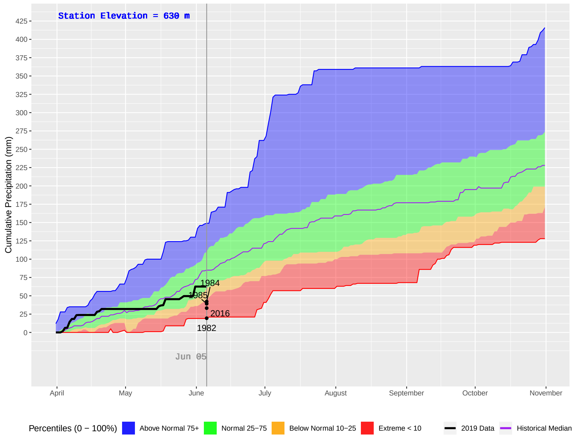
GRAND FORKS (392) : Historical (1981–2018), Current (2019) Daily Cumulative Precipitation
