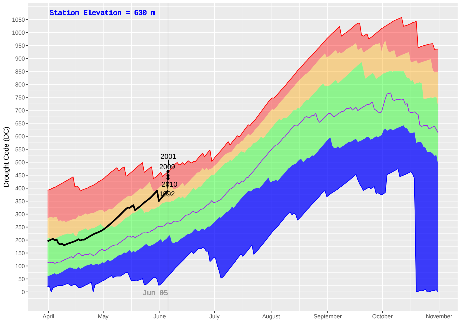
GRAND FORKS (392) : Historical (1981–2018) and Current (2019) Daily Drought Code (DC)
