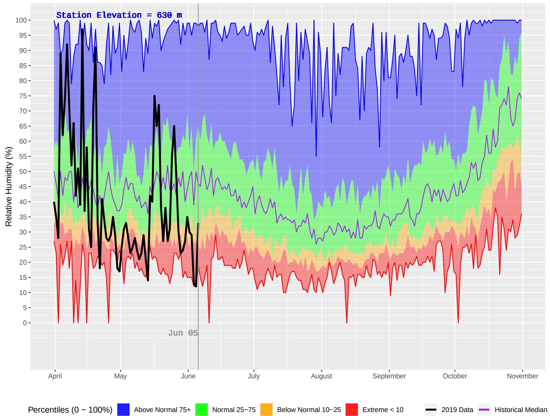
GRAND FORKS (392) : Historical (1981–2018) and Current (2019) Daily Relative Humidity
