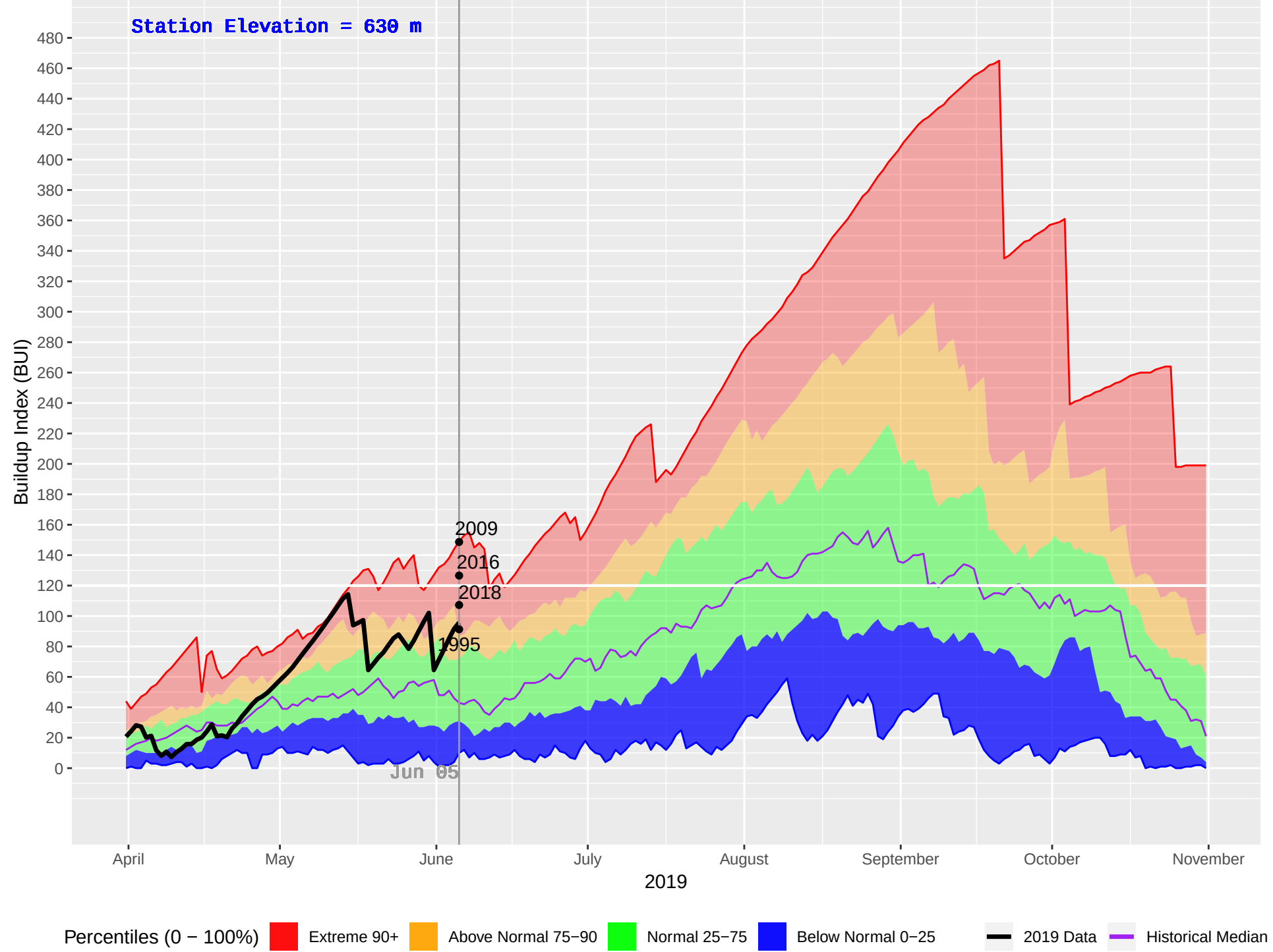
GRAND FORKS (392) : Historical (1981–2018), Current (2019) Daily Buildup Index (BUI)
