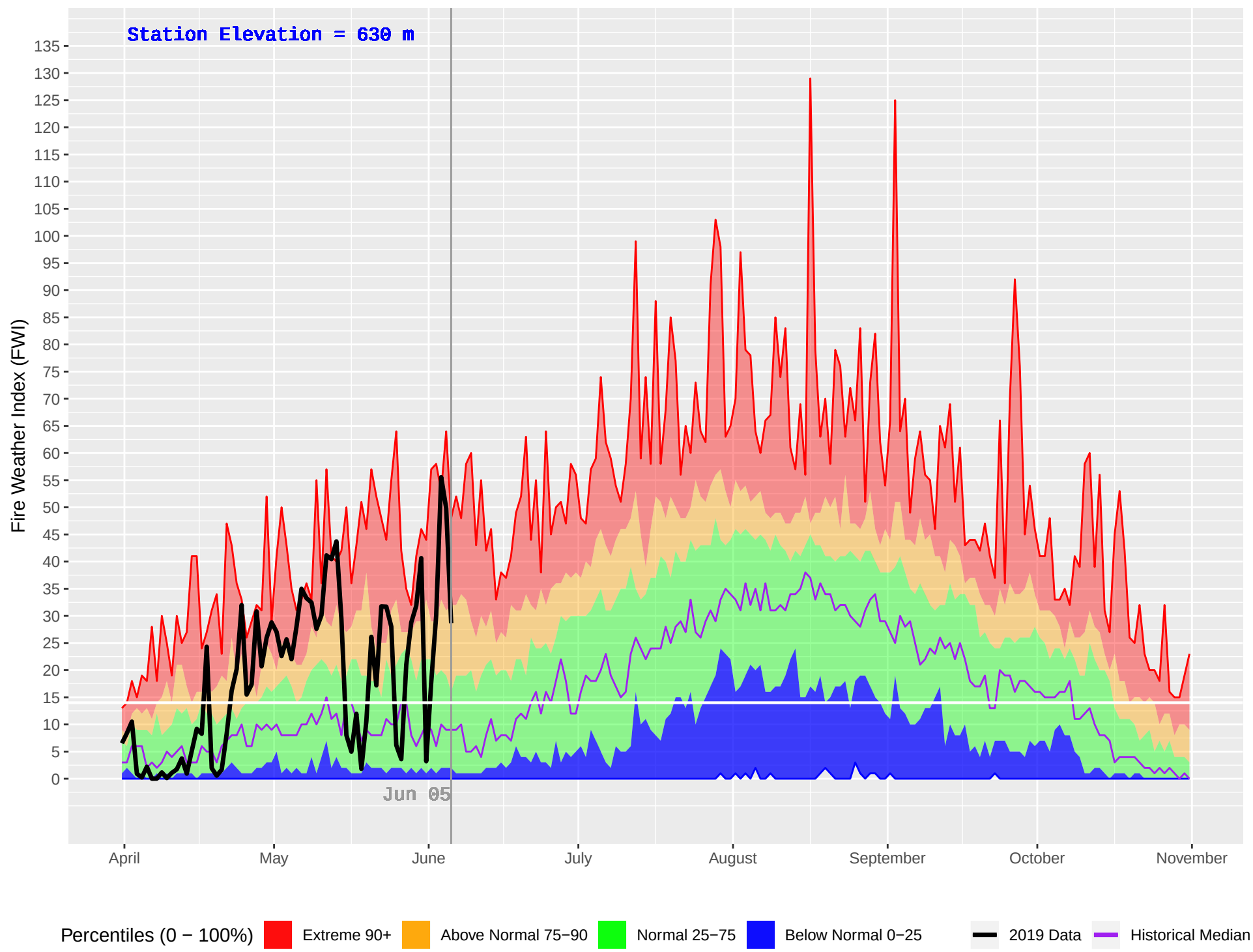
GRAND FORKS (392) : Historical (1981–2018) and Current (2019) Daily Fire Weather Index (FWI)
